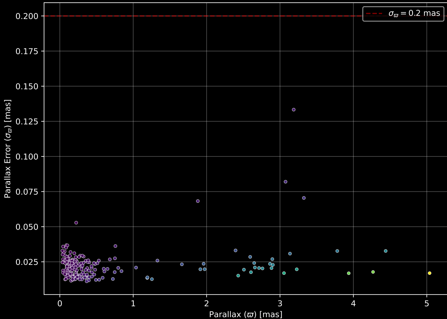
APOGEE DR17 Field: [049+12] Parallax Quality (n= 217)
