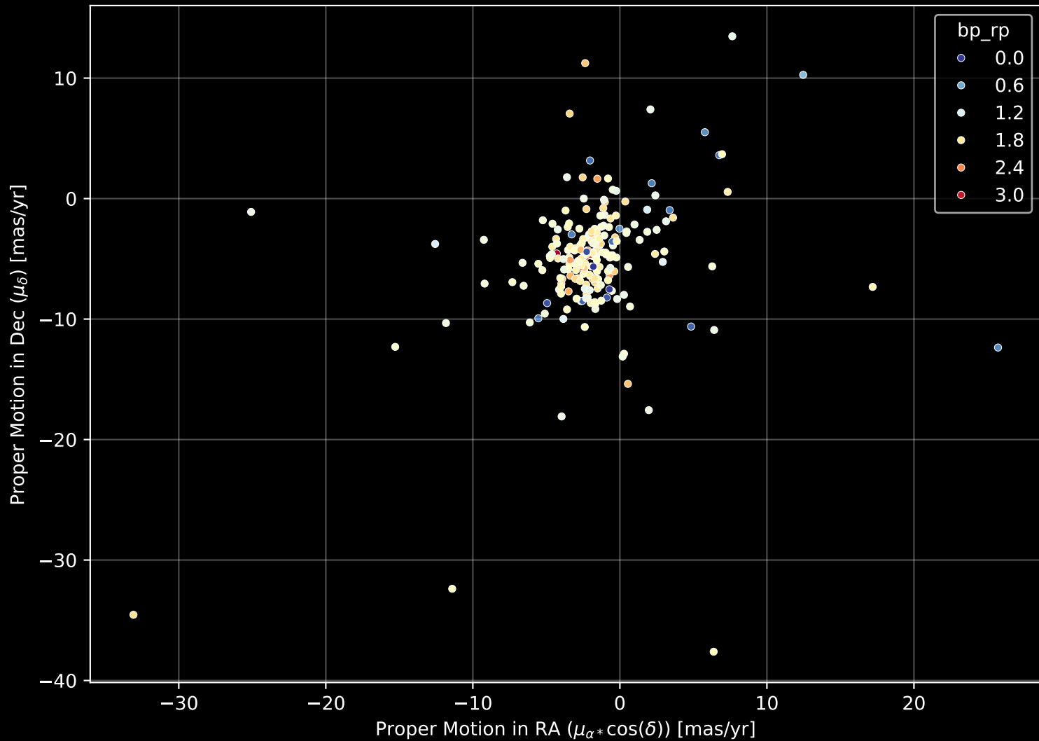
APOGEE DR17 Field: [049+12] Proper Motion Diagram (n= 217)
