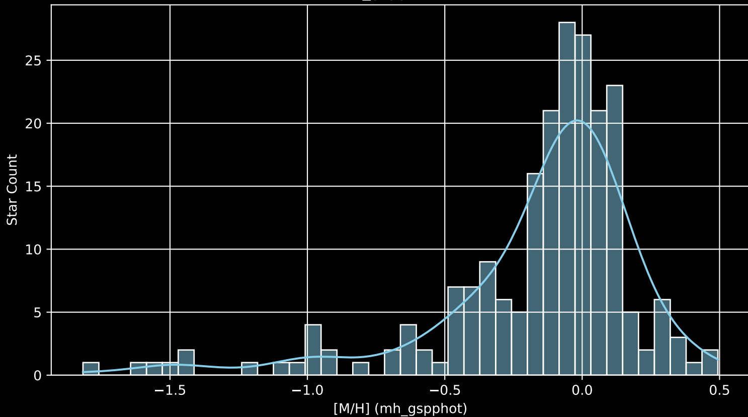
APOGEE DR17 Field: [049+12 [M/H] (mh_gspphot) (n= 214)
