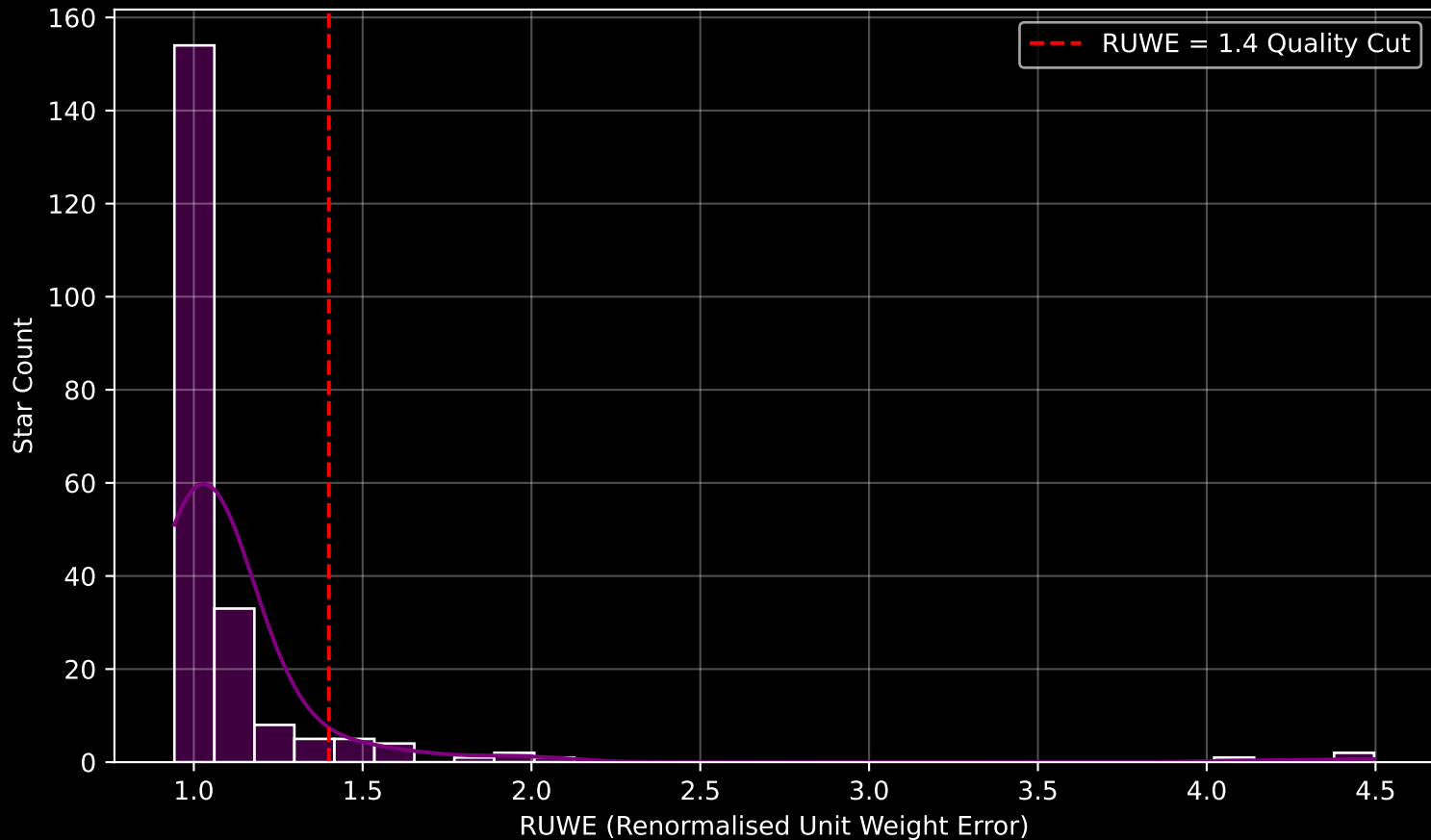
GAPOGEE DR17 Field [049+12] RUWE Distribution (n= 216)
